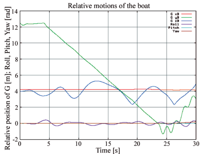
Fig. 8. Linear and angular motions of the lifeboat. Ship side's coordinate system. Diagram of the relative motions of lifeboat's mass centre and the lifeboat rotations: roll, pitch, yaw
