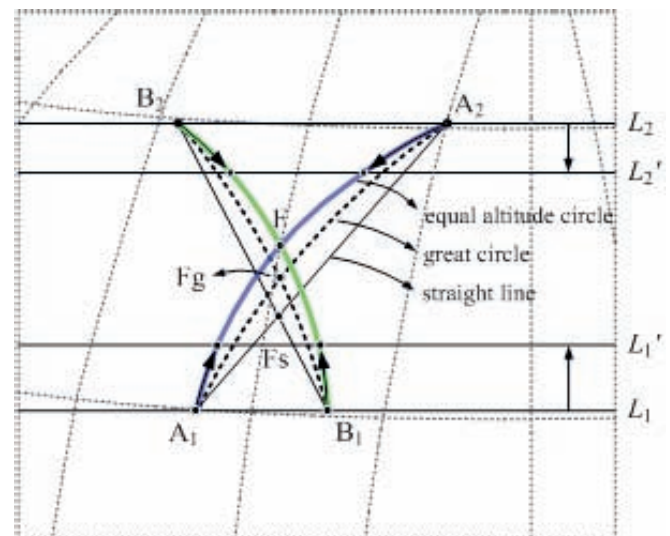
Fig. 2. Illustration of iteration scheme
