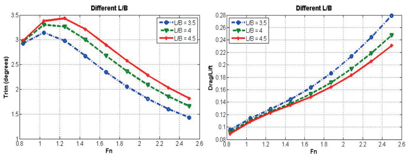
Fig. 6. The variation of trim and \frac{Drag}{Lift} ratio in function of Froude number F_n for three \frac{L}{B} values
