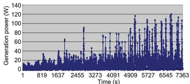
Fig. 10. Generation power distribution in 2013
