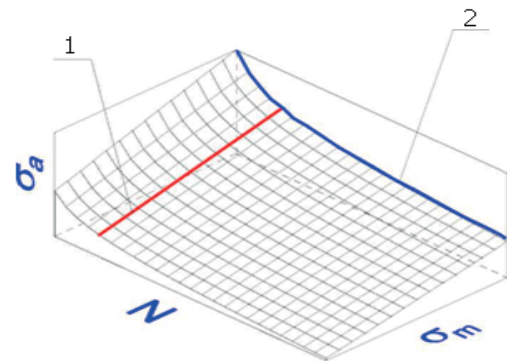
Fig.5 Limiting surface of variable stress amplitudes as function of the number of cycles N and the average stress value \sigma_m , \sigma_a = f(N, \sigma_m) . Curves 1 and 2 show trends of \sigma_a changes in N and \sigma_m directions [7 and 8].
