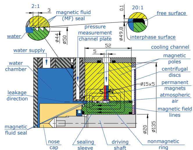
Fig.1. The examined MF sealing system with three teeth.
