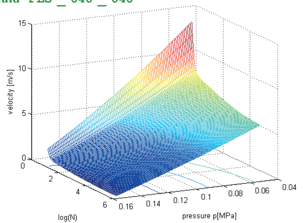
Fig.12. Experimental relation between the number of revolutions N until leakage and the circumferential velocity v of the seal, for different water environment pressures p . The number of revolutions shown in the \log N form. Magnetic fluid in the seal: FLS040.040 [5].
