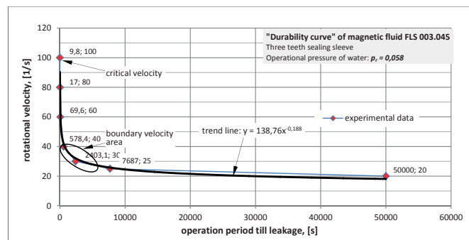
Fig. 3. Durability of seal with magnetic fluid FLS 003.045 in contact with water vs. rotational speed of sealing sleeve. The sealing system is shown in Fig.1
