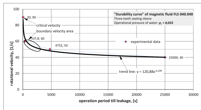
Fig. 4. Durability of seal with magnetic fluid FLS 040.040 in contact with water vs. rotational speed of sealing sleeve. The sealing system is shown in Fig.1 FLS 040.040. p_r = 0,053
