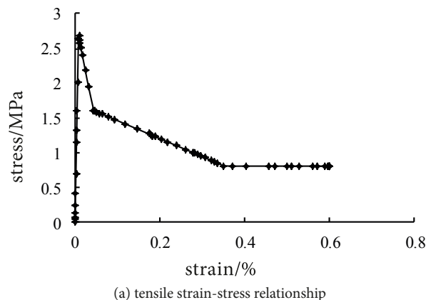
(a) tensile strain-stress relationship
