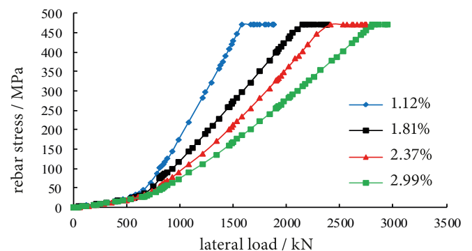
Fig. 8. Effect of reinforcement ratios on the stress of rebar
