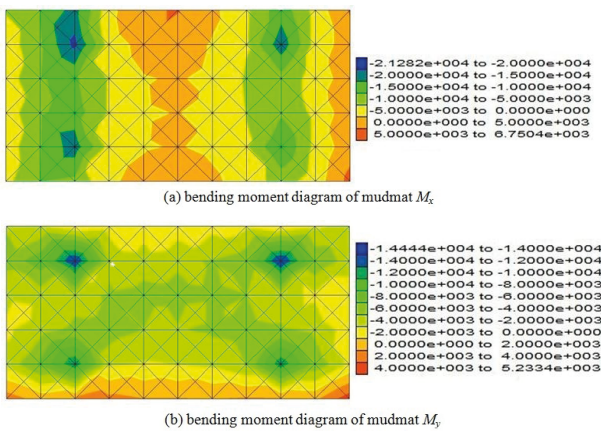
Fig. 14. Bending moments of the mudmat (unit: N·m)
