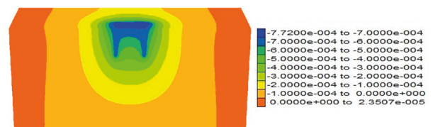
Fig. 7. Settlement of the seabed soil (units: m)
