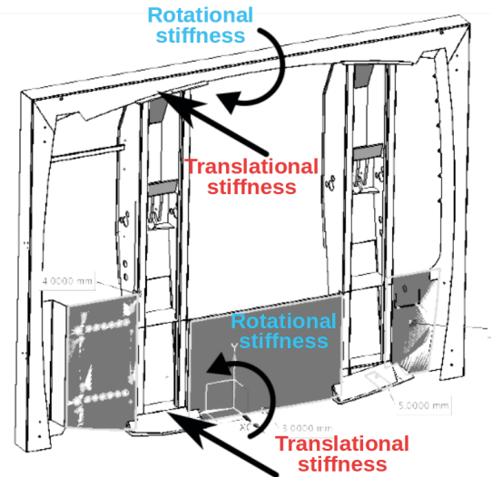
Fig. 8. Interpretation of the boundary conditions with regard to the stiffness of support provided by frame
