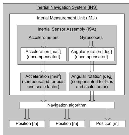
Fig. 2. Classification of inertial systems
