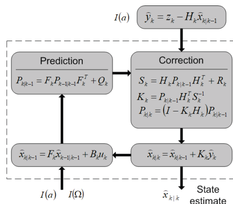
Fig. 3. Kalman filtering algorithm
