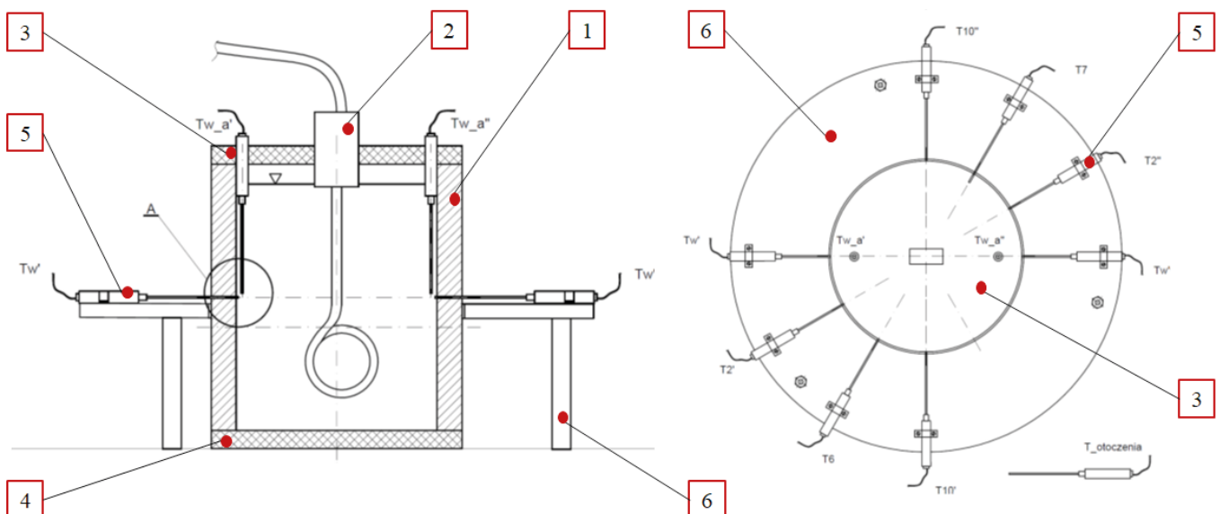
Fig. 8. Test stand for examining heat exchange through bush wall; 1 – tested bush, 2 – electric heater of 300 W power, 3 – cover (PMMA), 4 – bottom (PMMA), 5 – thermocouples K \varnothing 1 mm, 6 – sensor support
