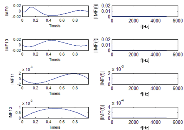
Fig. 12 9–12-dimension IMF and Corresponding Frequency Spectrums
