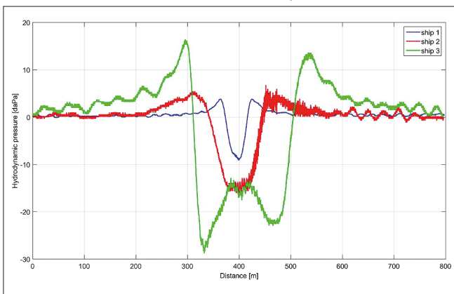
Fig. 8. Hydrodynamic pressure changes for three floating objects at speed 3.5 m/s (vessel 1 with length 60 m, vessel 2 with length 150 m, vessel 3 with length 230 m) for sea condition 1–2.
