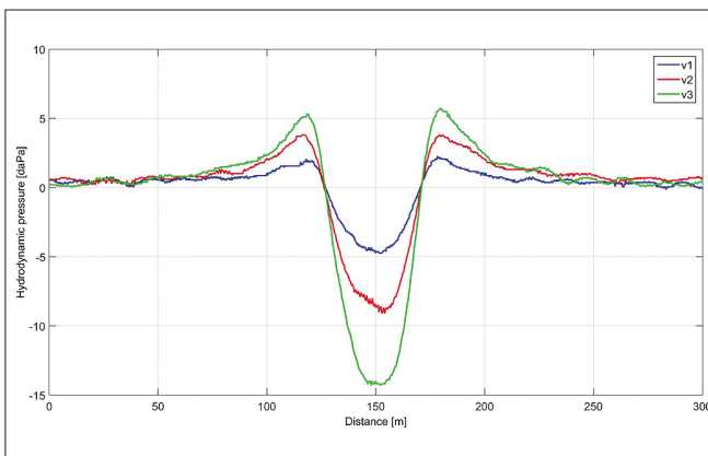
Fig. 9. Hydrodynamic pressure values for different speeds of the same vessel (v1 – 2.5 m/s, v2 – 3.5 m/s and v3 – 5 m/s) for sea condition 1–2
