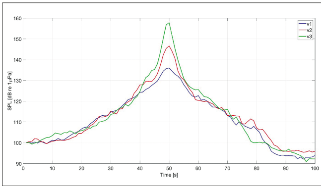
Fig. 7. Hydroacoustic pressure values for different speeds of the same vessel (v1 – 2.5 m/s, v2 – 3.5 m/s and v3 – 5 m/s) for sea condition 1–2
