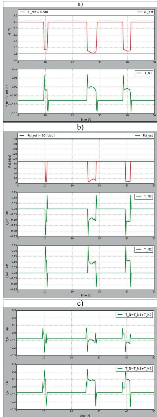
Fig. 15. Control time waveforms of the OpenROV collision avoidance process for the set reference distance d_{ref} = 0.5 m and fixed orientation \psi_{ref} = 90^\circ
