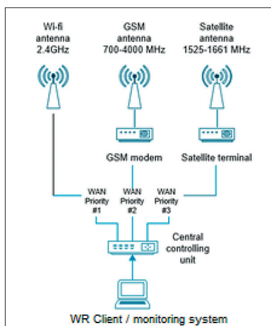
Fig. 6 Key elements of the hybrid communication system
