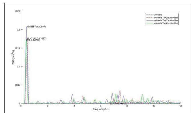
Fig. 6. PSD of the tower surge motion under different wave heights
