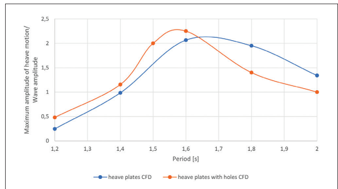
Fig. 8. Maximum amplitudes of heave motion
