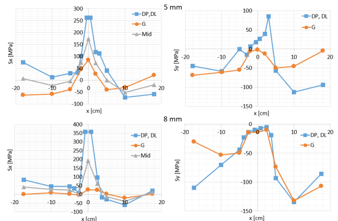
Fig. 3. Welding-induced residual stresses, plate element of 5 mm (top) and 8 mm (bottom) thickness
