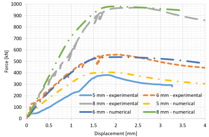
Fig. 11. Force-displacement relationship of 5, 6, and 8 mm specimens
