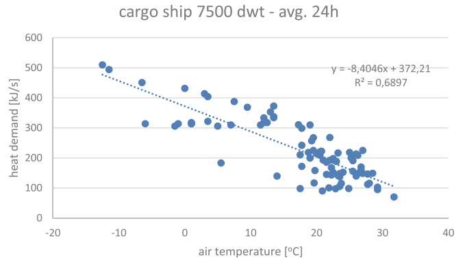
Fig. 5. Chart Q_{CE} = f(t_{air}) for ships; a) container ship 5300 TEU, b) cargo ship 7500 dwt
