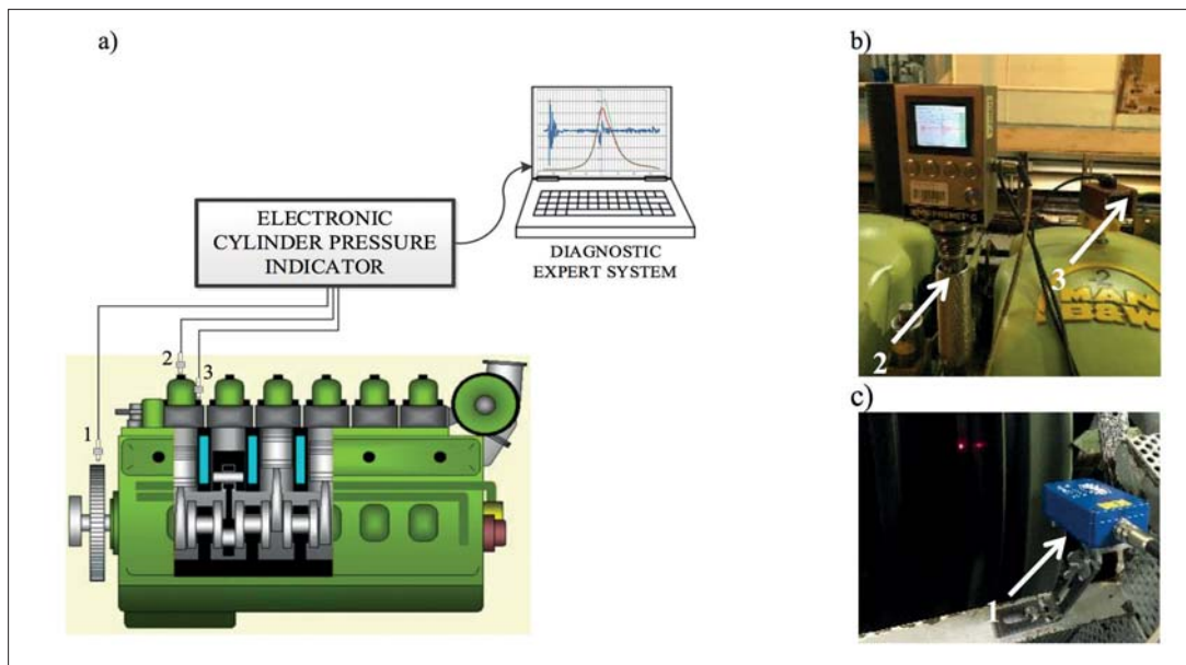
Fig. 4. Elements of the system diagnosing the working spaces of a marine engine by means of an electronic cylinder pressure indicator: a) schematic diagram; b) method of mounting the electronic indicator of the LEMAG PREMET C type (along with a pressure transducer) on the indicator cock and the vibration acceleration transducer on the nut fixing the head cover (from the inlet valve side); c) method of mounting the laser sensor of the rotational speed of the engine output's shaft. 1 – angular position sensor of the crankshaft; 2 – cylinder pressure sensor; 3 – vibration acceleration converter [6]
