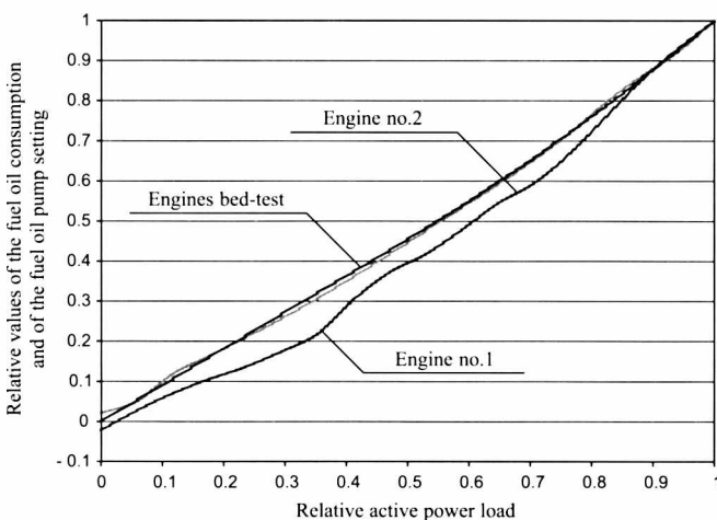
Fig.1. Relative values of the fuel oil consumption and relative settings of the fuel oil pump indices of the electric generating sets in function of the relative active power load of the electric generators
