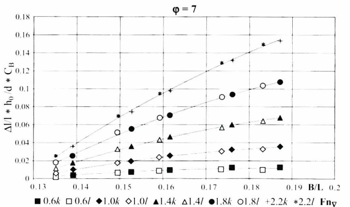
Fig. 9. The diagram of the coefficient (\Delta l/l * h_0/d * C_B) = f(B/L) for \varphi = 7
