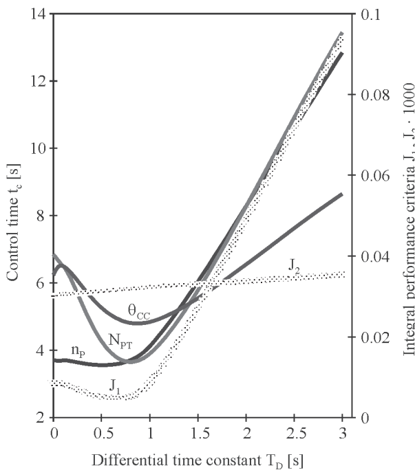
Fig. 14. The integral control performance criteria J_1 and J_2 and the ship propulsion system control time t_c in function of the controller settings k_p and T_D at step changes of the propeller pitch ratio H/D , determined for the following parameters of the ship propulsion system: n_p , N_{PT} , \theta_{CC} . Controllers with limiters; calm sea conditions
