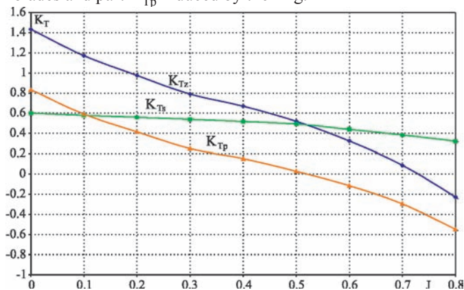
Fig. 3. Approximate division of total thrust K_{Tz} into part K_{Ts} induced by thruster blades and part K_{Tp} induced by the surrounding ring (nozzle).
