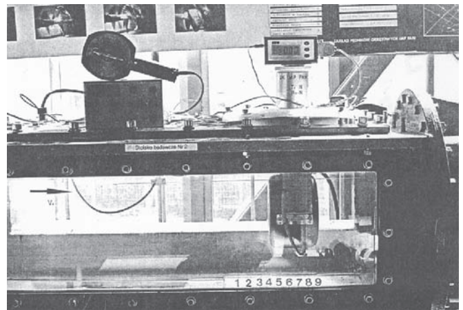
Photo 1. Research rig for ring thruster examination.
