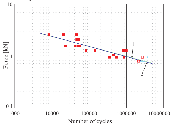
Fig. 7. Fatigue life diagrams of B_3 elementary structures .
