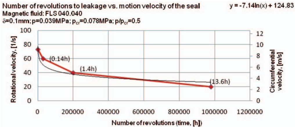
Fig. 5. Life of the seal with the applied FLS 040.040 magnetic fluid for the gap height of 0.1 mm and the set pressure of 0.039 MPa
