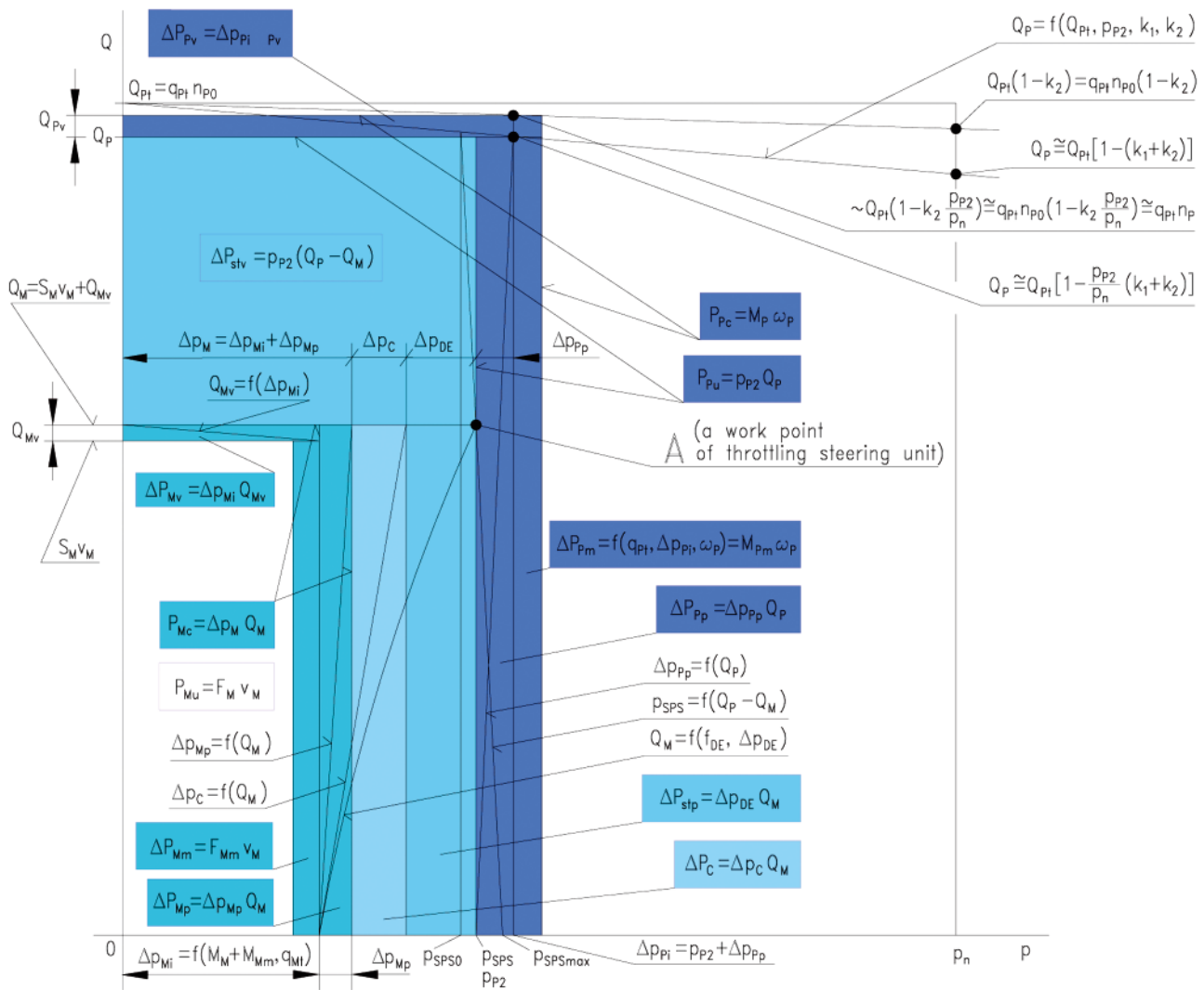
Fig. 3. Graphical interpretation of the power of losses in the hydrostatic drive and control system elements. An individual system with series throttling control of the hydraulic linear motor speed, fed by a constant capacity pump cooperating with the overflow valve in a variable pressure system – p = \text{var} ; the series throttling control assembly in the form of [3]: - adjustable throttling valve (together with a controlled overflow valve, creating a three-way flow regulator); - servovalve; - proportional directional valve
