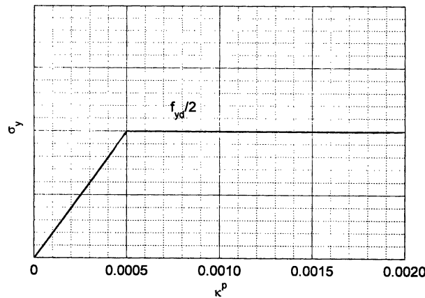
Figure 3. Equivalent yield strength function \sigma_\gamma versus second invariant of the deviatoric deformation tensor \kappa^p assumed for reinforcement ( f_{\gamma d} – yield stress)
