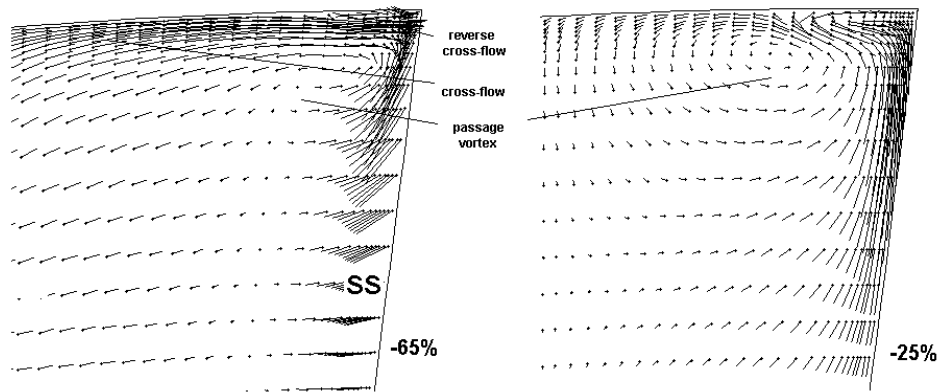
Figure 27. Secondary flow vectors in the second stator 65% and 25% axial chord upstream of the trailing edge; SS – suction surface
