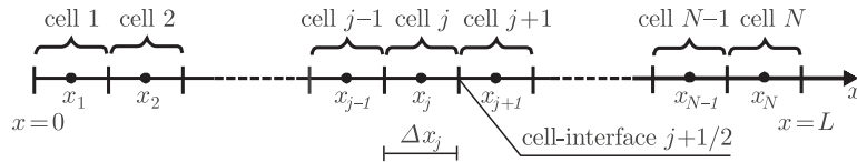
Figure 5. Discretization of the one-dimensional domain
