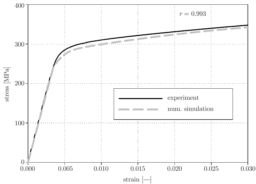
Figure 12. Results of B-P simulation of the uniaxial tension test for \dot{\epsilon} = 1 \cdot 10^{-3} \text{ s}^{-1} , for the specimen along the rolling direction of the sheet
