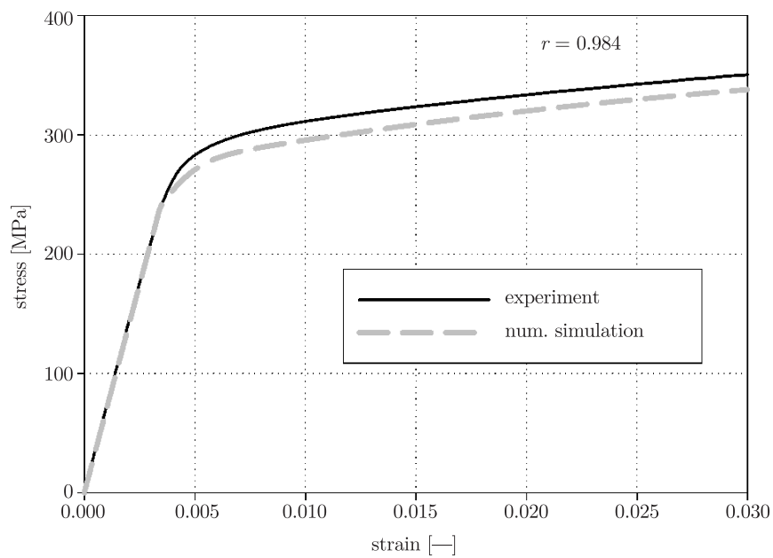
Figure 10. Results of B-P simulation of the uniaxial tension test for \dot{\epsilon} = 1 \cdot 10^{-4} \text{ s}^{-1} , for the specimen cut along the rolling direction of the sheet
