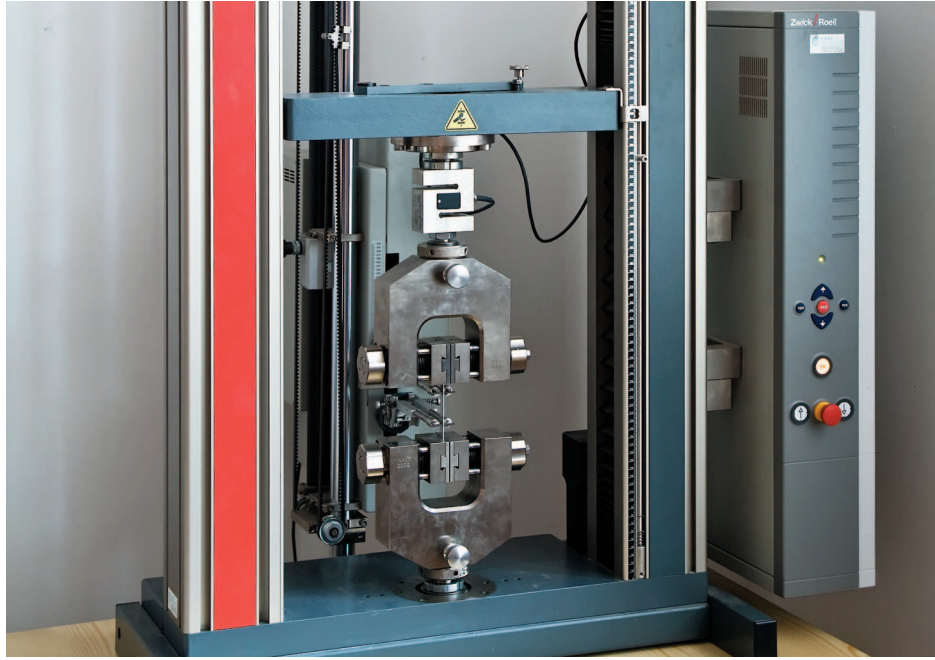
Figure 1. Experimental stand
