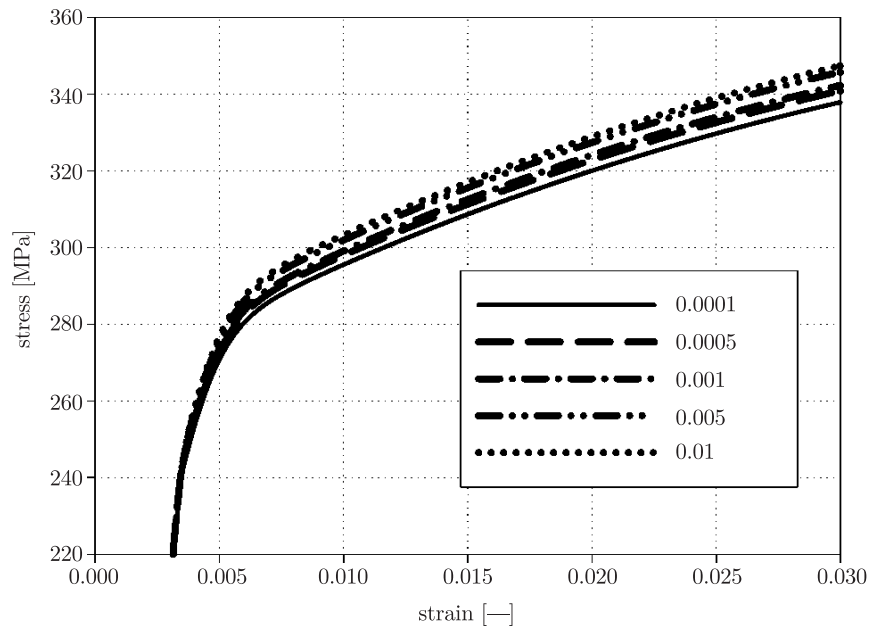
Figure 16. Results of B-P numerical simulation of the uniaxial tension test, inelastic range
