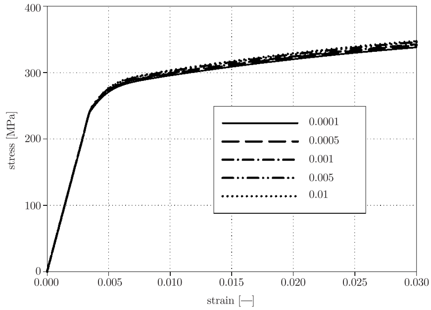
Figure 15. Results of B-P numerical simulation of the uniaxial tension test
