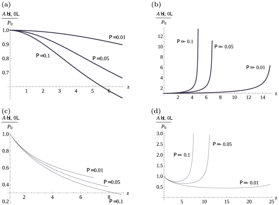
Figure 2. Dimensionless magnitude of acoustic pressure at the beam axis, A(z, r=0)/P_0 in a solitary shock wave (a,b) and in a monopolar impulse (c,d) (established by the first and second equations from the set Equation (27)-(28)) at different \Pi = \pm x_s/x_d . Positive \Pi corresponds to waveforms with positive acoustic pressure, and negative \Pi corresponds to waveforms with negative acoustic pressure. z = x/x_s designates the dimensionless distance from the transducer
