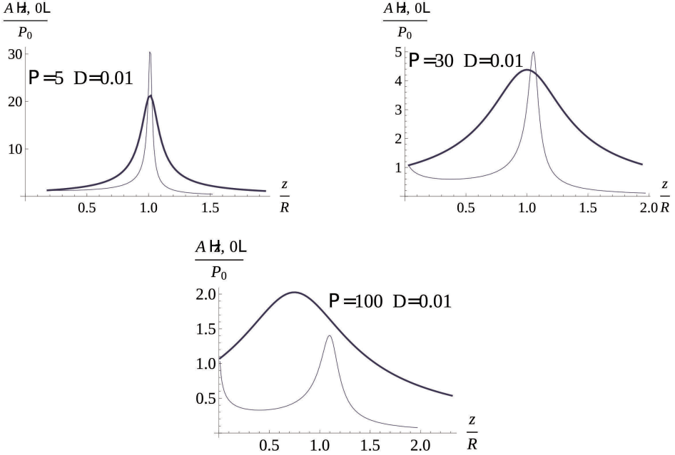
Figure 1. Dimensionless magnitude of acoustic pressure at the beam axis, A(z, r=0)/P_0 , as a function of the dimensionless distance from the transducer, z/R . The bold lines relate to the solutions of the first equation from the set Eq. (21)-(22) for a solitary positive shock, and the thin lines relate to the solutions of the second equation from the set Eq. (21)-(22) for a single positive impulse, which is triangular at the transducer, for different \Pi = R/x_s and D = R/x_d = 0.01
